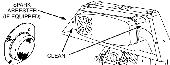
Muffler and Spark Arrester
